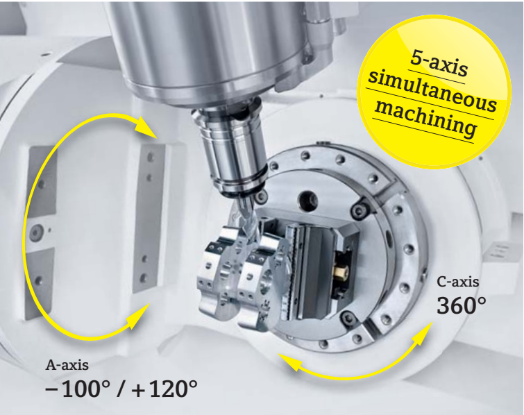
NEW: 12,000 rpm. inline spindle (in combination with a SIEMENS 840D solutionline control)
